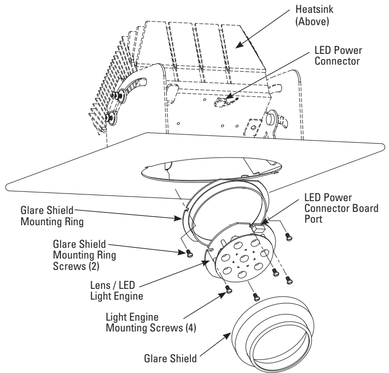
EXPLODED VIEW
